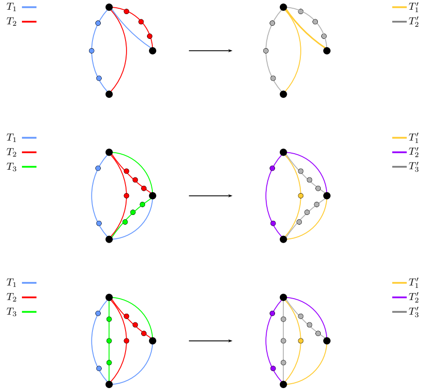
Figure 1: It can be considered that there exist at most two special \{x, y, z\} -trees in a connected graph with girth at least five and 3-connectivity at least two.
