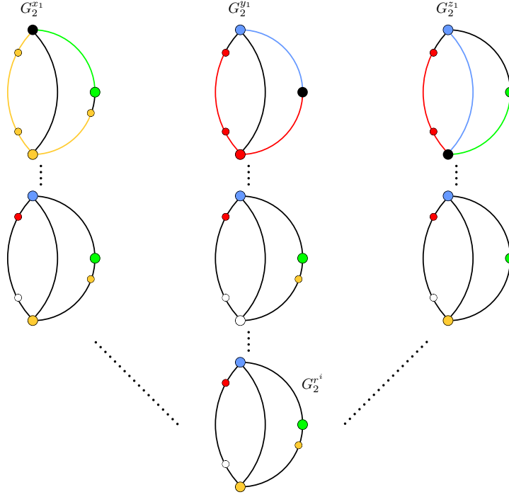
Figure 11: Four \{x, y, z\} -trees in G_1 \boxtimes G_2 associated to a path P_1 in G_1 and to special trees Q_1, Q_2 in G_2 .
