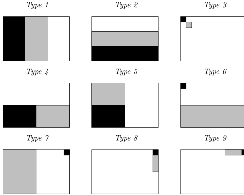
Figure 2: All possible types of minimum edge 3-cuts in G \square H .
