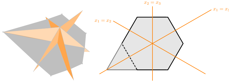
Figure 3: Generalized permutohedron
