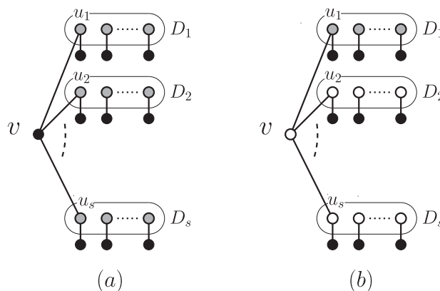
Figure 4. (a) Black vertices are in S . Black and gray vertices are in S^* . (b) There is a perfect dominating set not containing white vertices.
