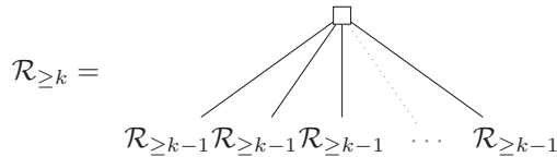
Figure 1: Symbolic equation for \mathcal{R}_{\geq k} .
