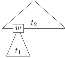
Figure 2: Decomposition at a k -protected vertex.
