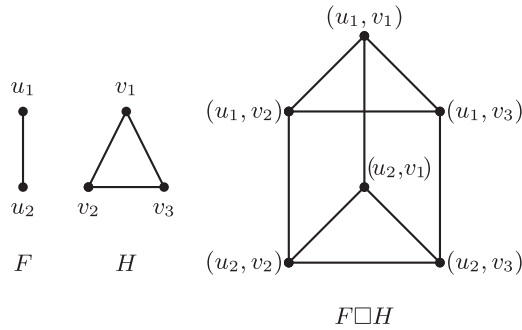
Figure 1. Cartesian product
